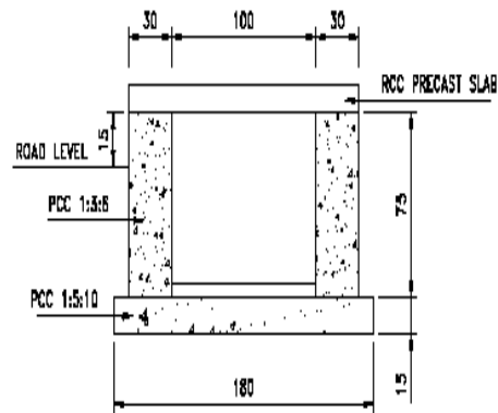
C.S. OF U DRAIN
