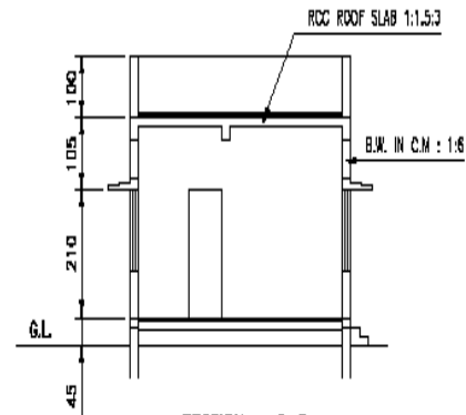
SECTION - 2-2
