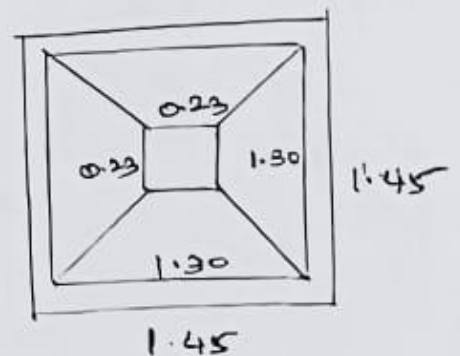
KARUMATHI SHED FOOTING PLAN
