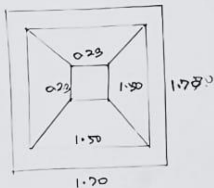
A. HIGHWADI CENTER FOOTING PLAN
