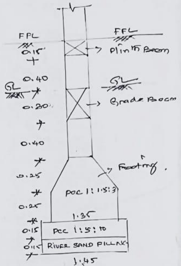
SECTION
