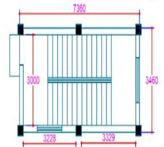
HEAD ROOM PLAN
