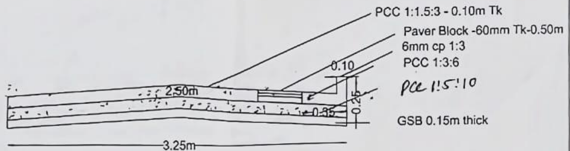
C/S OF CEMENT CONCRETE ROAD
