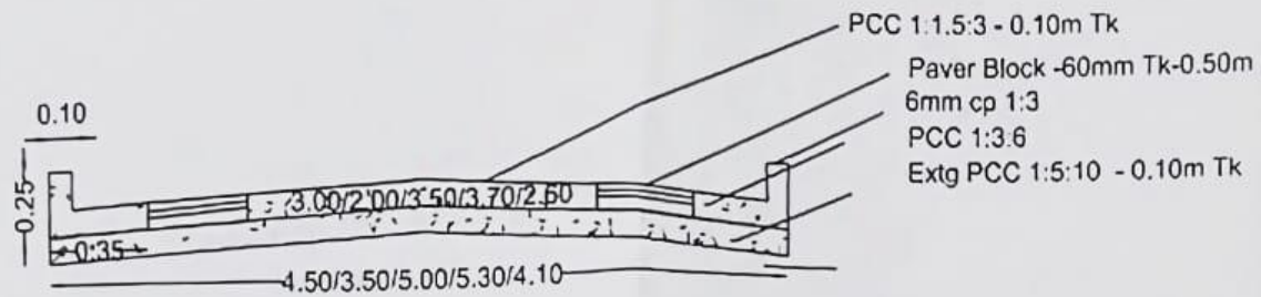
C/S OF CEMENT CONCRETE ROAD
