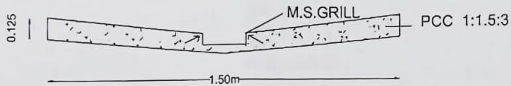
C/S of Causeway
