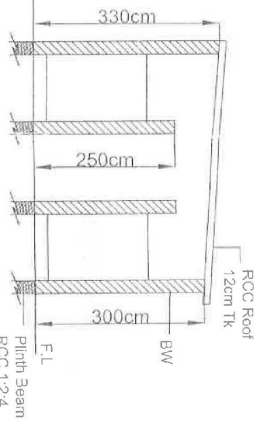
CROSS SECTION ON 'AA'
